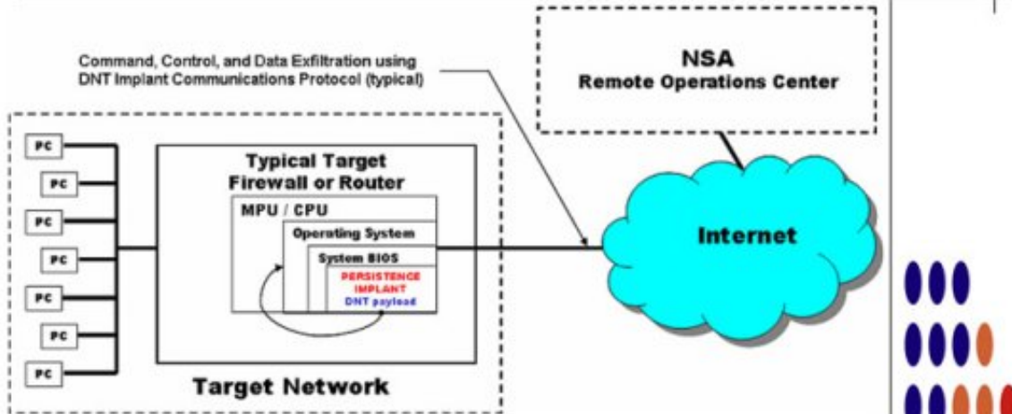
(S//SI//REL) STUCCOMONTANA Concept of Operations
