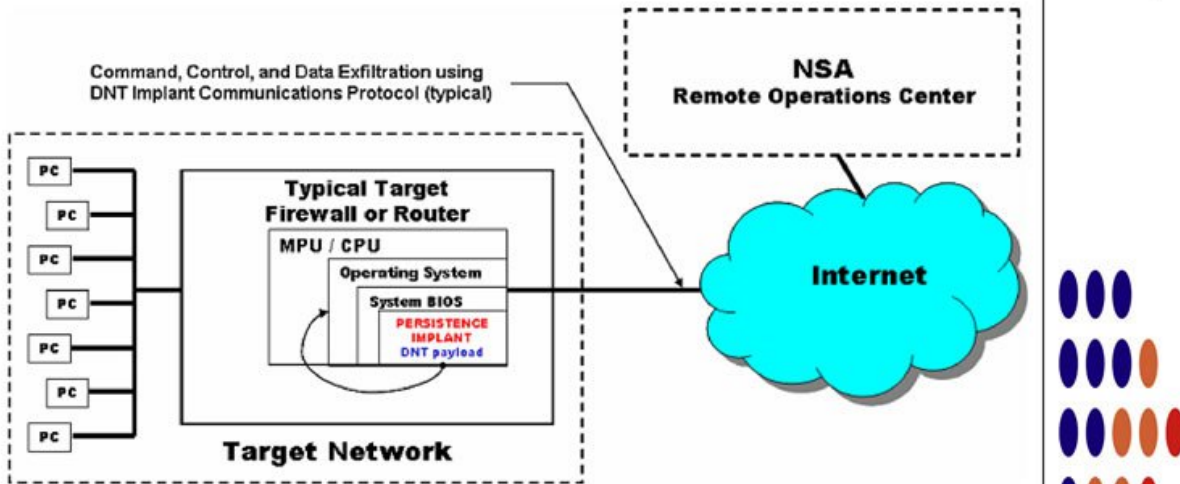
(TS//SI//REL) HALLUXWATER Persistence Implant Concept of Operations
