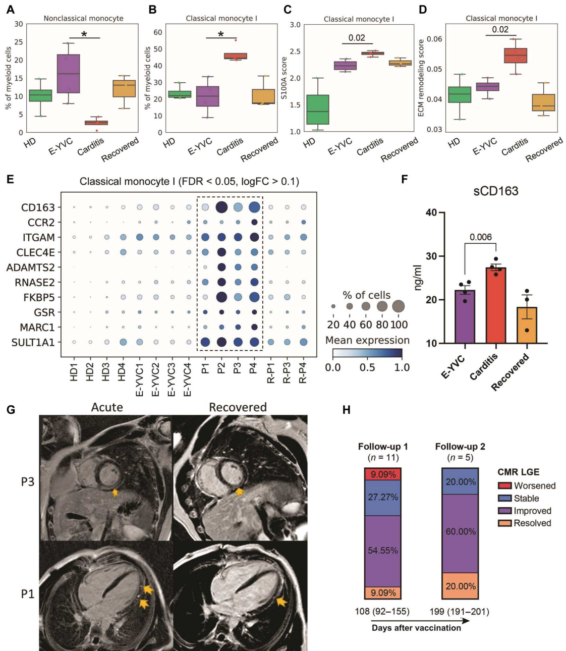
Fig. 5. Inflammatory and profibrotic signatures of monocytes in myopericarditis. (A and B) Box plots showing the average proportions of nonclassical (CD14 dim CD16 + ) and classical (CD14 + CD16 - ) monocyte subsets across the groups. The boxes denote the IQR, horizontal bars represent the median, whiskers extend to 1.5 × IQR, and dots show the values of each donor. Statistical significance was determined using the Bayesian model sCODA (49) accounting for the compositional dependencies between cell subsets in the scRNA-seq data while controlling for false discoveries (FDR < 0.05 in myopericarditis versus E-YVCs). (C and D) Average expression scores of (C) inflammatory genes from the S100A family of alarmins ( S100A8-12 ; FDR < 0.05, logFC > 0.1 in myopericarditis versus E-YVCs) and (D) 238 genes from a published dataset of extracellular matrix (ECM) remodelling (GSEA MSigDB M3468) in the same classical monocyte subset shown in (B) across groups. Statistical significance between scores was determined using the unpaired two-sided Wilcoxon rank-sum test comparing the E-YVC and myopericarditis groups. (E) Dot plot showing top differentially expressed and up-regulated genes in the same classical monocyte subset shown in (B) across donors (FDR < 0.05, logFC > 0.1 in myopericarditis versus E-YVCs). (F) ELISA measurement of sCD163 in serum across the groups. Statistical significance was determined using the unpaired two-tailed t test between the E-YVC and myopericarditis groups, and error bars represent the SE. (G) Representative CMR images of acute myopericarditis and follow-up/recovery (191 days for P1 and 82 days for P3 after vaccination) showing persistent LGE (yellow arrows) seen in a subset of patients (from 17 patients included in our cohort, at admission, 11 were LGE positive, 4 were LGE negative, and 2 had no CMR). Particularly, for P1, four-chamber phase sequence inversion recovery (PSIR) demonstrating patch subepicardial LGE along the left ventricular lateral wall from base to apex (acute), with improvement in both quantity and intensity at follow-up (recovered). For P3, mid-ventricle short axis PSIR demonstrating subepicardial to nearly transmural LGE sparing the subendocardial region (acute), which was mildly improved in intensity and quantity at follow-up (recovered). (H) Stacked bar plots depicting the percentage of patients categorized by CMR LGE changes at two follow-ups after vaccination/first admission [median days (IQR)]. Additional details of imaging findings and patients with LGE at admission and follow-up are in table S1.
