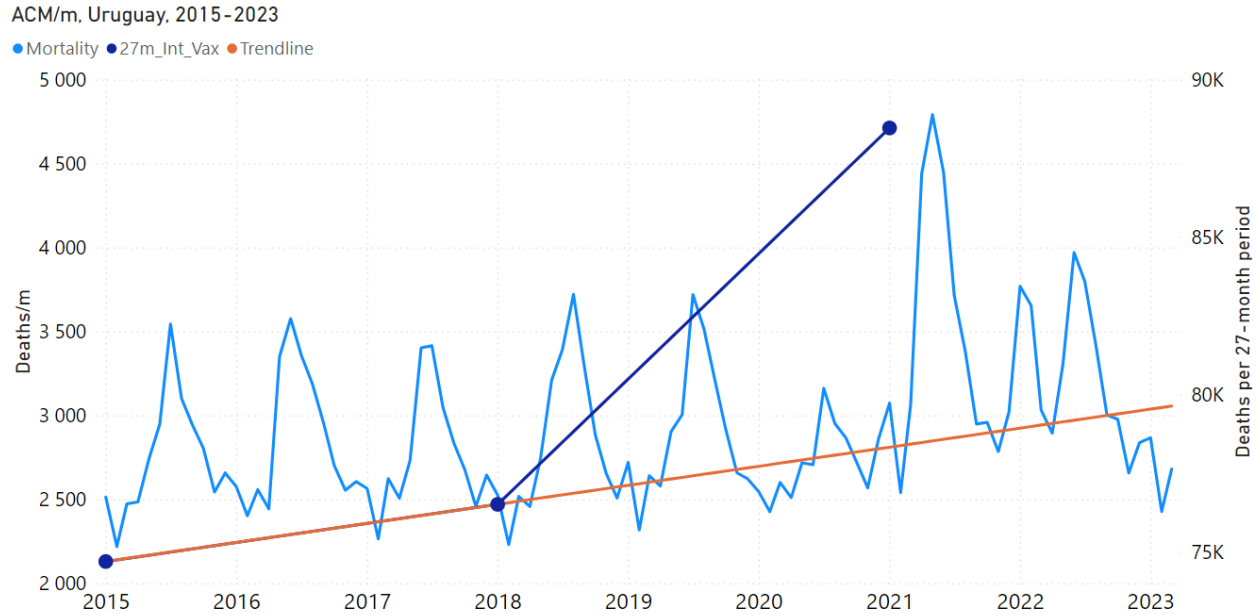
Figure 7: All-ages ACM by week (ACM/w) or by month (ACM/m) (light blue), 2015-2023, with integrations (dark blue), and trend lines (orange), for the for the vaccination period, for the 17 countries in this study (as labelled). The data sources are specified in Appendix A.
