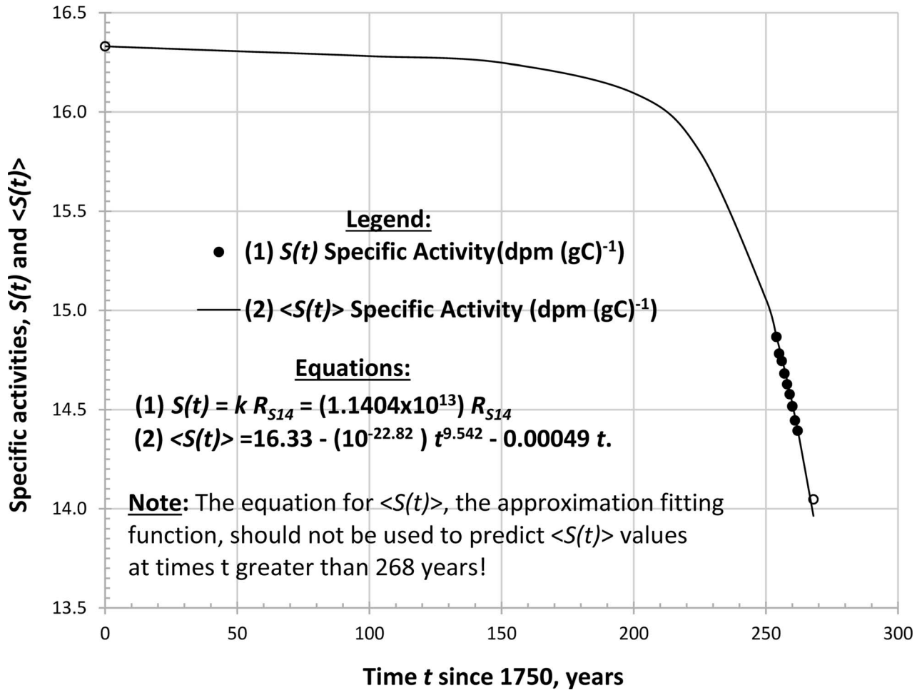
Fig. 2. Niwot Ridge, Colorado annual mean specific activity, S(t) , and expected specific activity, \langle S(t) \rangle , of 14 C in C(t) in 1750 through 2018.
